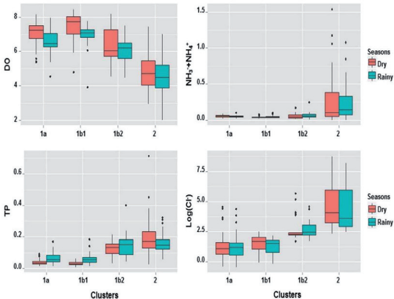
Fig 6. Seasonal variations between the dry (in red) and rainy (in blue) seasons for dissolved oxygen (DO), total phosphorus (TP), total ammonia ( \text{NH}_3 + \text{NH}_4^+ ) and chloride (Cl) within the four identified clusters. Vertical axis indicates the concentration of DO, TP, total ammonia and Cl in logarithmic scale in \text{mgL}^{-1} .
